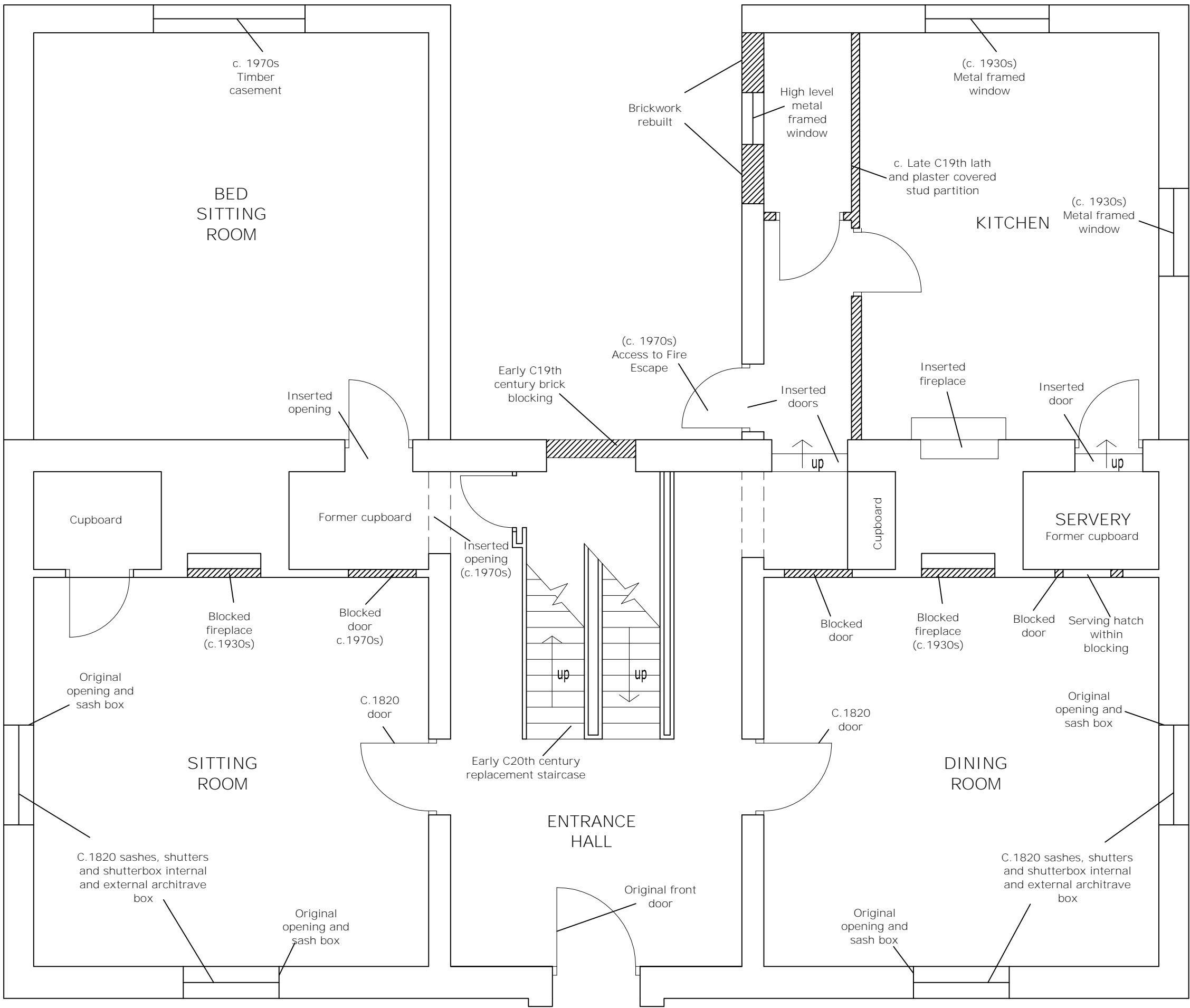
Figure 32: Walnut Tree House (B.30)) - upper ground floor plan
