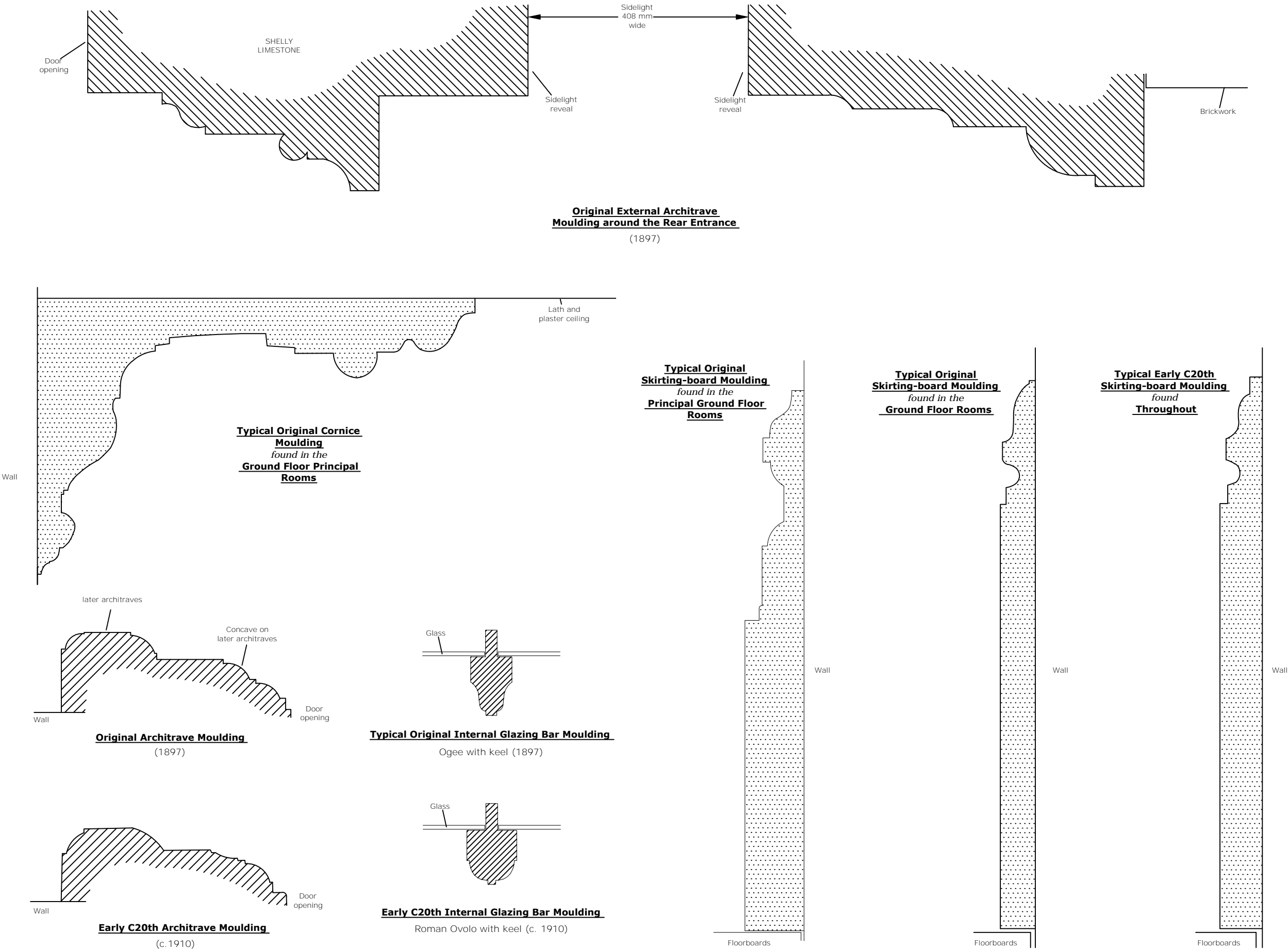
Figure 49: Mulberry House (B.43) - moulding profiles
